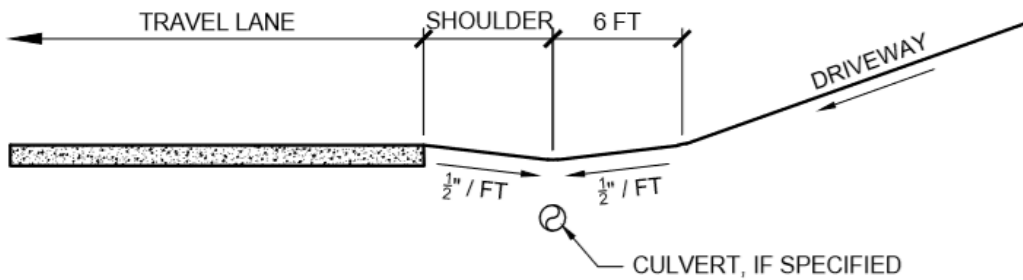
Profile of Driveway Downhill from Road
