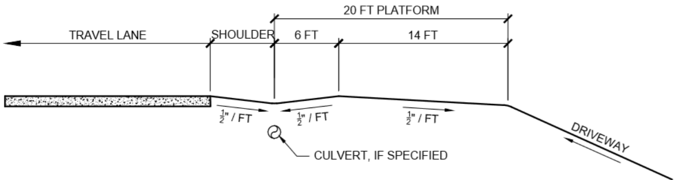
Driveway Cross Section
